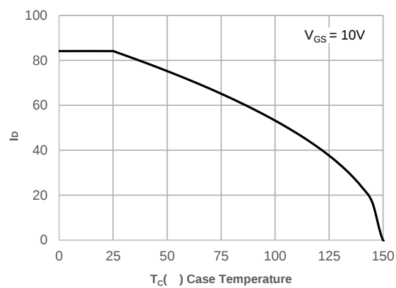
Figure 2: Current De-rating
